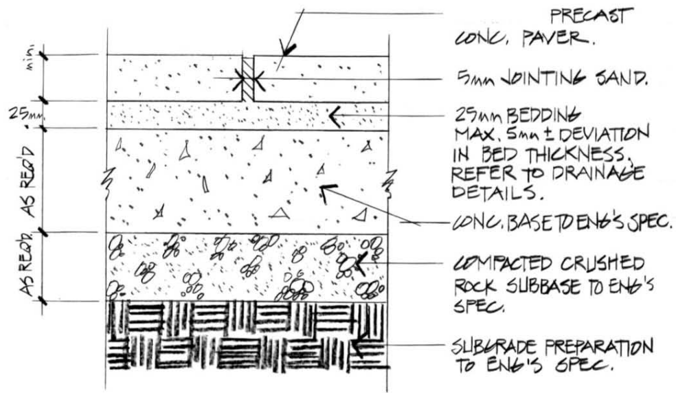
SECTION - VEHICULAR
